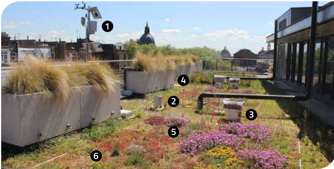
The roof is equipped with instruments to measure ① weather conditions ② rainfall ③ water quality ④ runoff ⑤ soil moisture ⑥ soil and roof temperature
